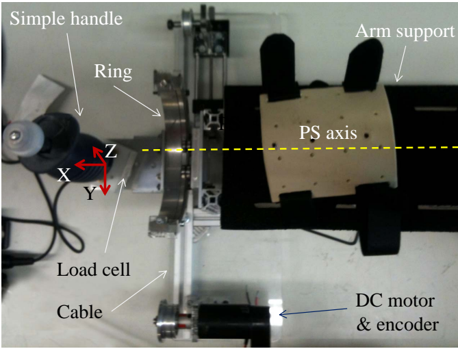
Fig. 1: The initial wrist robot to study the reaction forces during prono-supination rotation.
