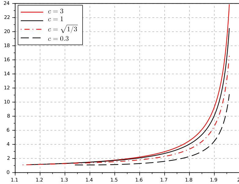
Figure 1 – Impact of the value of c on the function p \mapsto q_0 \Gamma(2 - p) .
