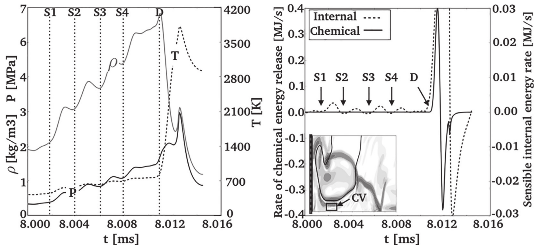
Fig. 15. Temporal evolution of key parameters integrated along the control volume (CV) shown on the right figure: (Left) Temperature, pressure and density; (Right) Chemical energy release rate and sensible energy release rate. S1 – 4 mark a series of four consecutive shock compressions. D marks the moment the mixture detonates.
