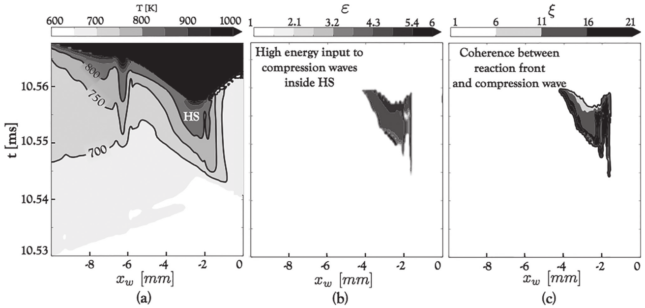
Fig. 14. Time evolution of temperature (a), \epsilon (b) and \xi (c) in the single-step case through the cut line presented in Fig. 10(Right), positioned 500 \mu m from the bottom wall. x_w is the distance from the obstacle 6 left wall. IS, RS, CS, R and D denote an incident shock, a reflected shock, a compression wave, the detonation wave, and the detonation wave, respectively. HS is a hot spot.
