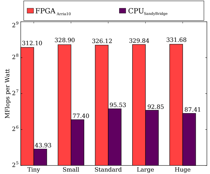
Fig. 5. Energy efficiency results.
