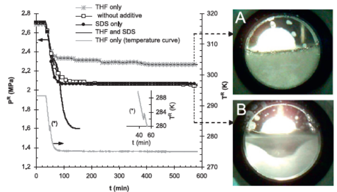
Fig. 7. Comparison of four different kinetic curves (reactor pressure and temperature versus time) obtained with and without additives. [THF] 4 wt%, [SDS] 0.3 wt%.
