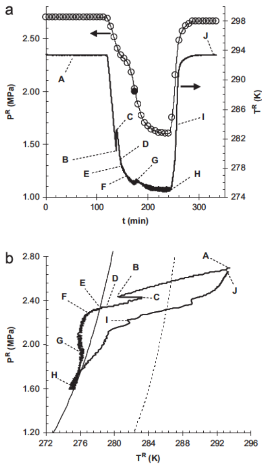
Fig. 6. Type curves corresponding to a \text{CO}_2 enclathration experiment carried out in batch configuration, initial reactor pressure 2.70 MPa, [THF] 4 wt%, [SDS] 0.3 wt%. (a): reactor pressure and temperature as a function of time ; (b) P - T diagram corresponding to the experimental data, the regular line is the \text{CO}_2 hydrate equilibrium pressure from CSMGem (Sloan and Koh, 2008), the dashed line is the \text{CO}_2 +THF mixed hydrate equilibrium curve (our data) obtained with [THF] 4 wt%.
