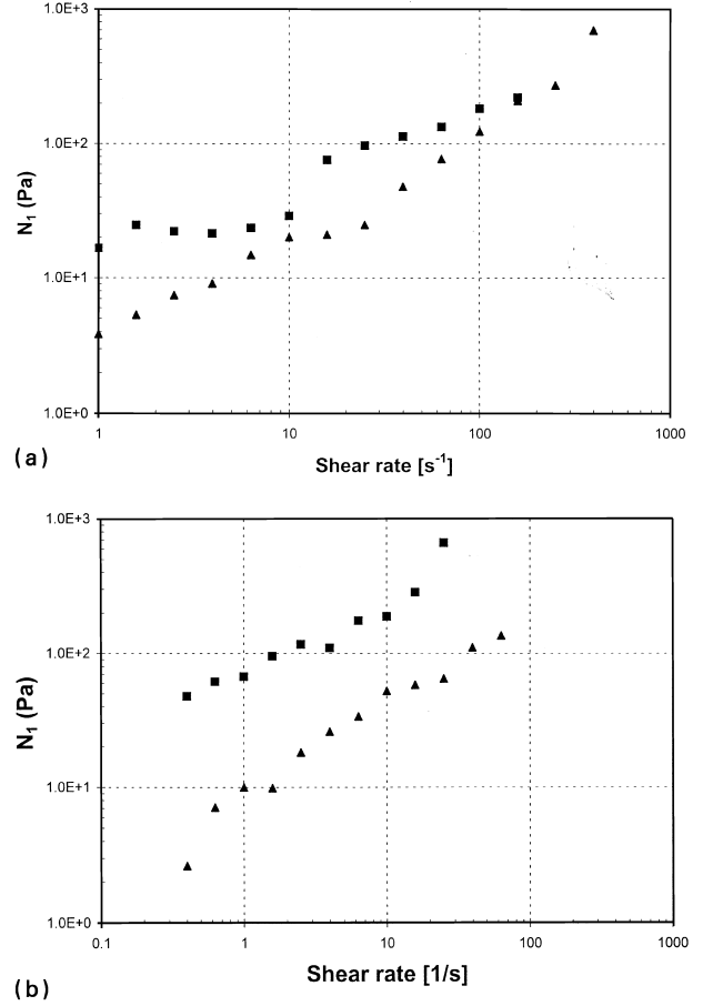
Fig. 8. (a) The first normal stress difference N_1 for PMMA in toluene with different molar mass. ■ M_w = 1.92 \times 10^7 g/mol. ▲ for M_w = 1.06 \times 10^7 g/mol. (b) The first normal stress difference N_1 for PMMA in DMF with different molar mass. ■ for M_w = 1.92 \times 10^7 g/mol. ▲ for M_w = 1.06 \times 10^7 g/mol.
