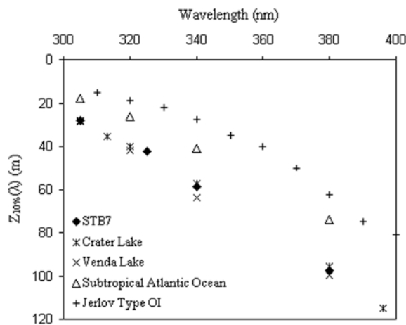
Figure 2. Z_{10\%}(\lambda) at 305 nm (UV-B), and 325, 340 and 380 nm (UV-A) determined between 0 m and 30 m in the hyper-oligotrophe zone of the South Pacific Gyre (STB7 station). For comparison, we reported Z_{10\%}(\text{UV}) values obtained for the clearest oceanic waters, i.e. the Jerlov Type OI waters [Jerlov, 1976; Smith and Baker, 1981] and the Subtropical Atlantic Ocean (23°N, 38°W) [Obernosterer et al., 2001], and for the clearest fresh waters, i.e. the Crater Lake (Oregon) [Hargreaves et al., 2007] and the Vanda Lake (Antarctic) [Vincent et al., 1998].
