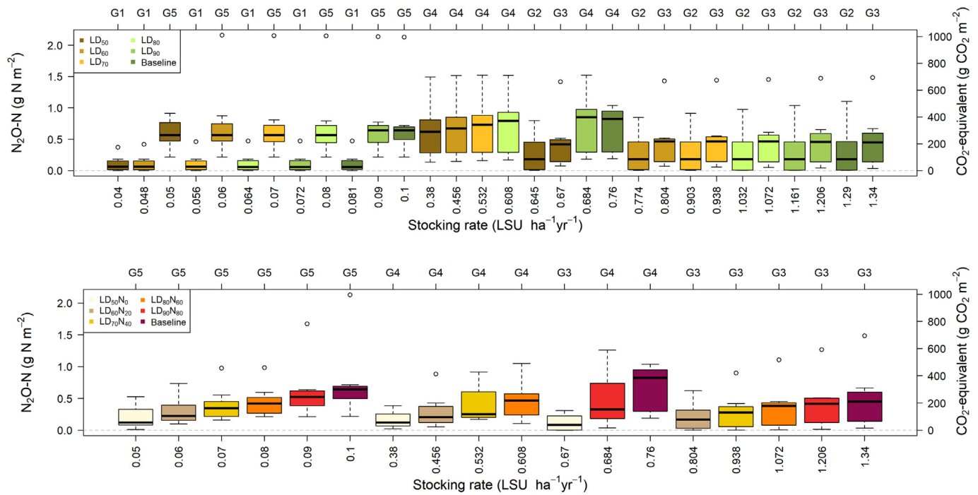
Fig. 4. Relationship between nitrous oxide emissions (multi-year averages of seven models) given in \text{N}_2\text{O-N} and \text{CO}_2\text{e} forms, and increasing animal stocking rate at all sites comparing livestock density reductions (top graph) and livestock density and N fertilization reduction (bottom graph), as in Table 3.
