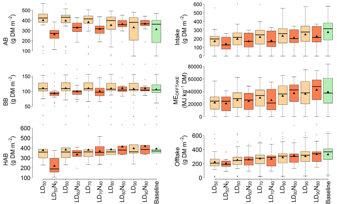
Fig. 6. Changes in productivity and energy outputs (g DM m -2 , MJ kg -1 DM) calculated over multiple years at five sites, for ten altered management scenarios and the baseline (as in Table 3). For each management level, triangles show the multi-model (as in Table 4) mean, black lines show multi-model median. Boxes delimit the 25th and 75th percentiles. Whiskers are 10th and 90th percentiles. Points indicate outliers.
