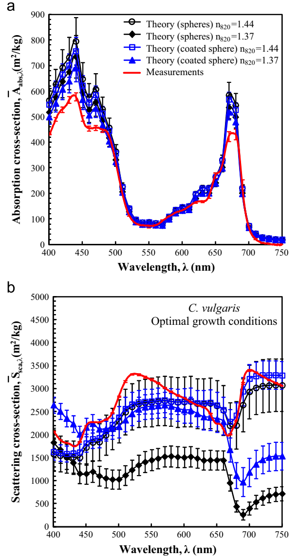
Fig. 6. Comparison between experimentally measured and theoretically predicted average spectral mass (a) absorption \bar{A}_{abs,\lambda} and (b) scattering \bar{S}_{sca,\lambda} cross-sections of C. vulgaris grown in optimal growth conditions. Theoretical predictions treated the cells as polydisperse spheres or coated spheres with n_{820} equal to 1.44 or 1.37.
