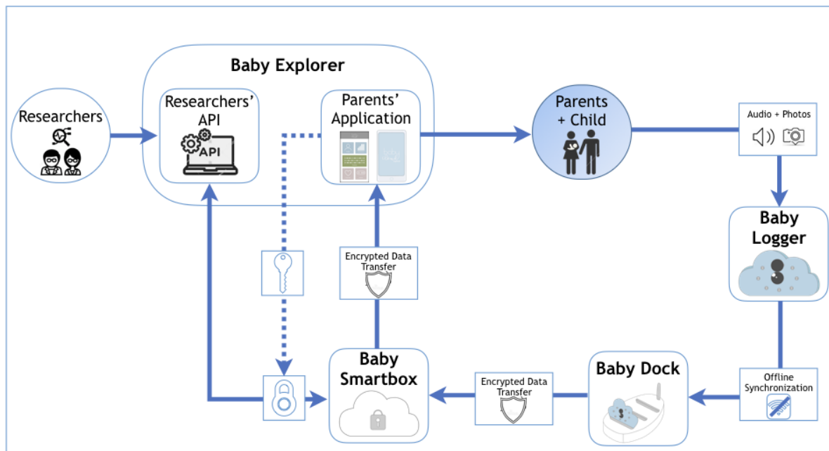
Figure 1: BabyCloud Workflow.
