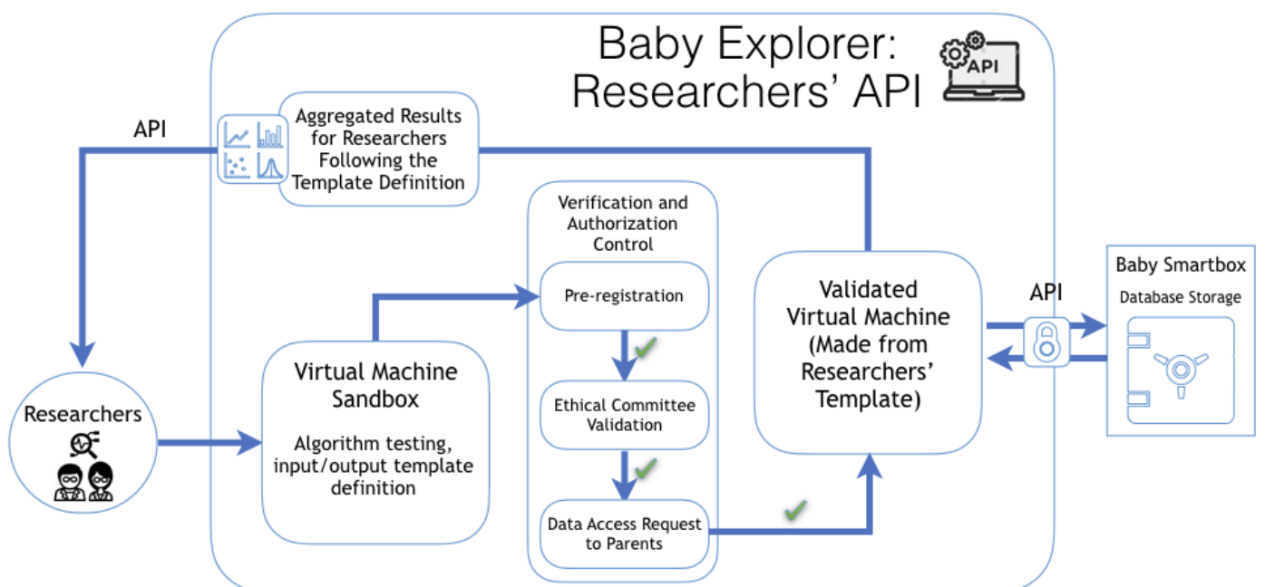
Figure 6: Baby Explorer Architecture: Researcher's API.
