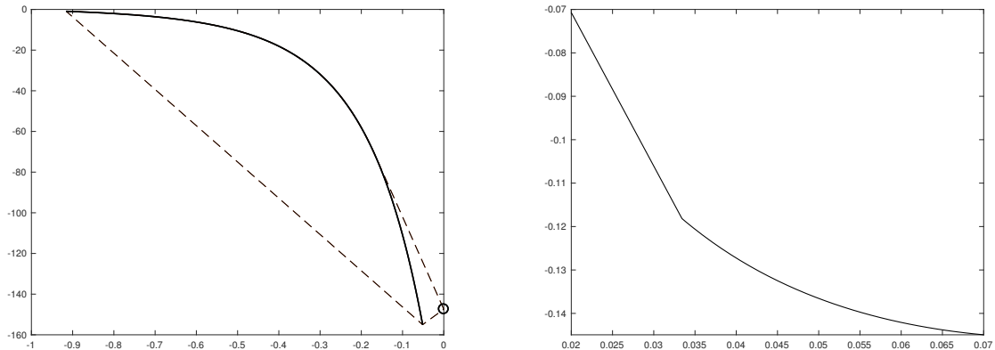
Figure 2: The set A on the left and the corresponding value function v = v_A in (22) for the insurance example on the right. Parameter values are \alpha = 0.08 , f = 10 , \varpi = 1000 , R = 10 .
