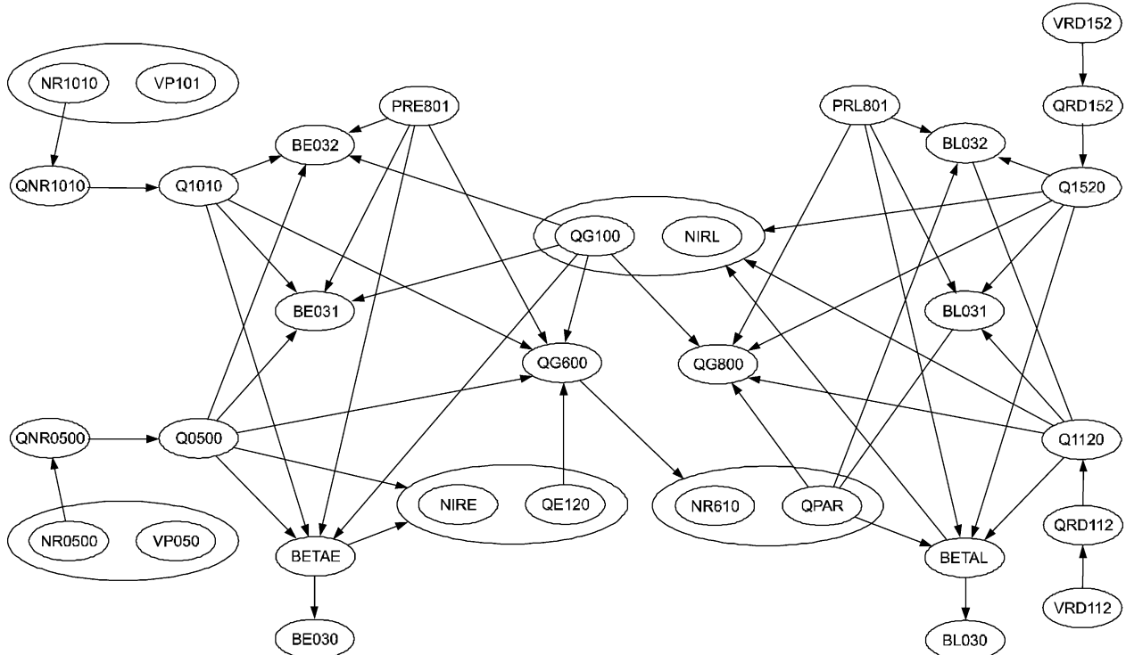
Fig. 13. Complete causal graph of the two columns.
