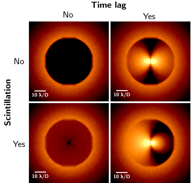
Fig. 3. Simulated images using HCIPy for the parameters gathered on Tab. 1. The images with no time lag were produced with an infinite AO loop speed. Only a time-lagged WDH and scintillation yields an asymmetric coronagraphic PSF. The images are purposely stretched in intensity to highlight the asymmetry and scintillation (log scale).
