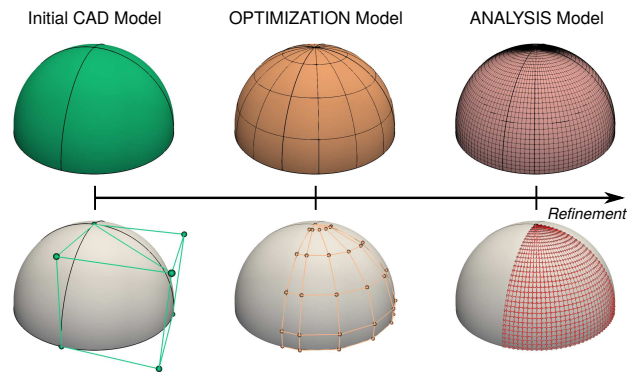
Fig. 2 Multi-level design approach: optimization and analysis spaces describe the exact same geometry and are initially obtained through different refinement levels of the CAD model (above: NURBS elements, below: control points).
