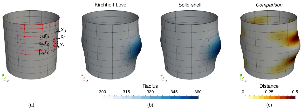
Fig. 6 Shape optimization of the pinched cylinder: (a) 6 design variables update the optimization model, (b) final shapes obtained by both shell formulations, and (c) comparison of the final shapes depicted as the distance between their mid-surface.
