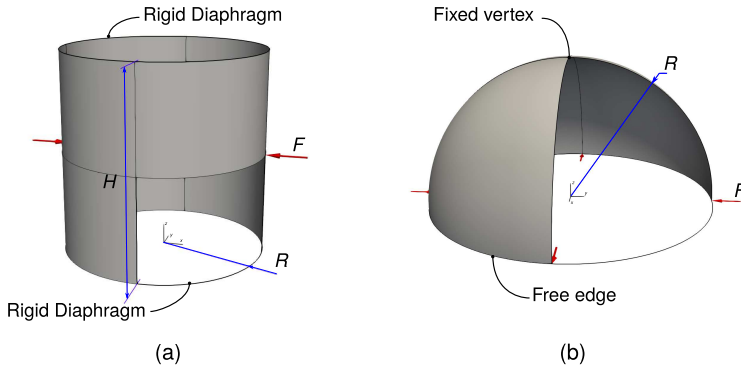
Fig. 5 Numerical examples to investigate the use of isogeometric solid-shell elements for shape optimization of shell structures: (a) pinched cylinder and (b) pinched hemisphere.
