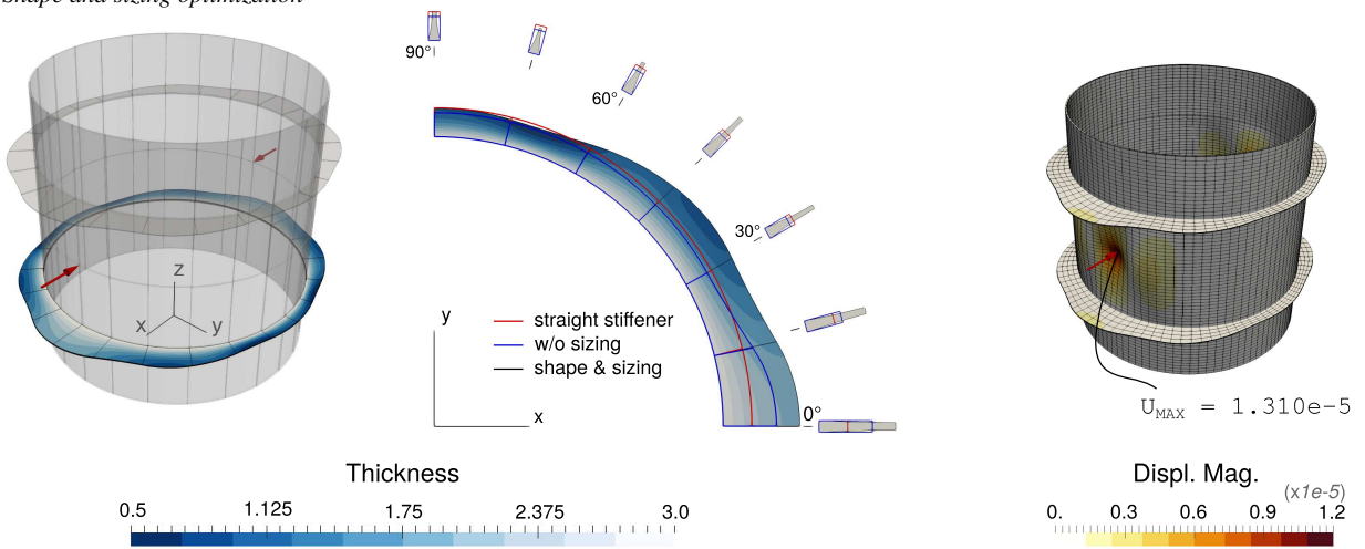
Fig. 11 Optimization results of the stiffened cylinder: (a) final shape when only the stiffener height is modified, and (b) final shape when both height and thickness are optimized. From left to right are depicted a general 3D view of the final shapes, a top view and several cross sections of the final stiffeners, and the displacement fields for these two optimized designs (annotations on figure 9 can be helpful to understand the detailed views of the stiffener).
