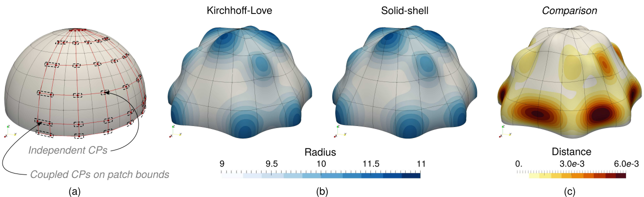
Fig. 7 Shape optimization of the pinched hemisphere: (a) 25 design variables update the optimization model, (b) final shapes obtained by both shell formulations, and (c) comparison of the final shapes depicted as the distance between their mid-surface.
