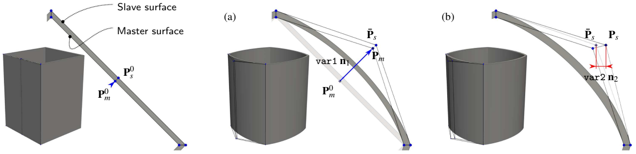
Fig. 4 Definition of the design variables in the context of solid-shell isogeometric elements. (a) A first set of design variables updates the master surface and (b) the slave surface follows the shape variation through a second set of variables.
