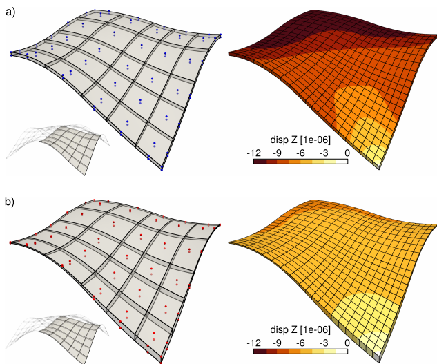
Fig. 15 Volume models of the roof: a) initial geometry and initial Z-displacement field, b) optimal geometry and its corresponding Z-displacement field.
