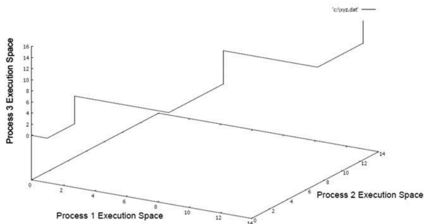
Lattice Chain for Cyclic Unreliable Unicast based Distributed Computing on 3-Manifold
