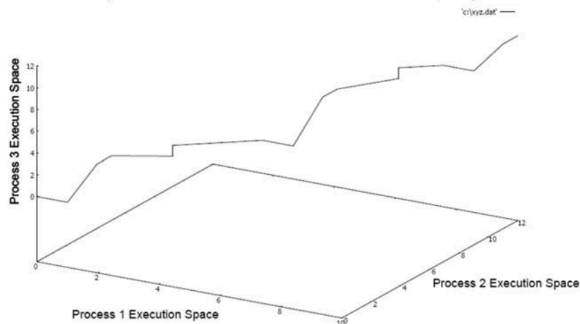
Lattice Chain for Cyclic Unreliable Broadcast based Distributed Computing on 3-Manifold
