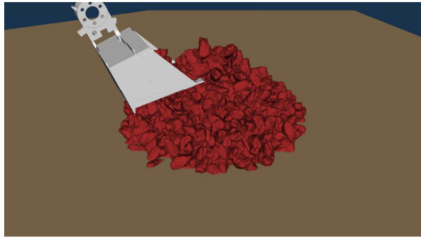
Fig. 18 The InSight scoop interacting with granular particles captured from three-dimensional X-ray computed tomography. The exact geometry of the scoop can be replicated in advanced DE Models. These methods can simulate different particle size distributions and particle shapes
