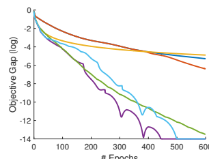
Figure 3: Lasso Regression on MARTI2 Dataset
