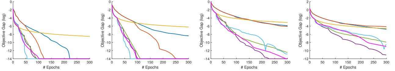
Figure 5: Lasso regression on Madelon dataset with additional random features ( A \in \mathbb{R}^{2000 \times 4000} )
