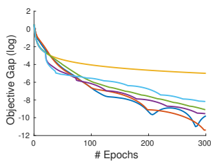
Figure 1: Lasso Regression on RCV1 Dataset
