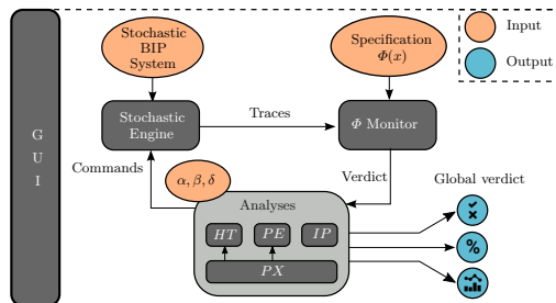
Fig. 1: SBIP architecture
