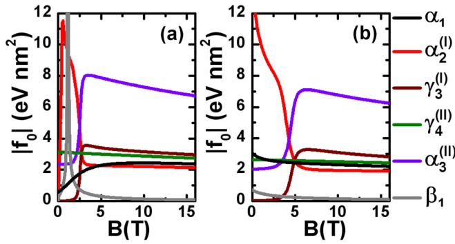
FIG. 3. Oscillator strength f_0 = \hbar^2 \overline{f_{\text{osc}}}/(2m_0) for Landau-level transitions shown in Fig. 2. The overline denotes an averaging over orientation of the light polarization lying in the QW plane. The (a) and (b) panels are connected with those in Fig. 2.
