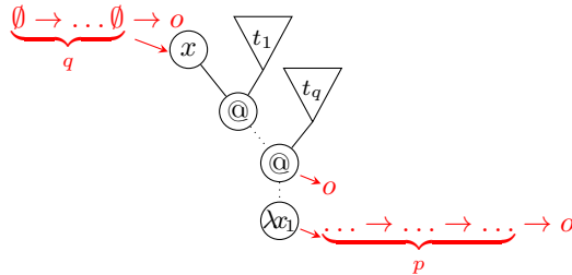
Figure 2: Typing a Head Normal Form in an i.t.s.
