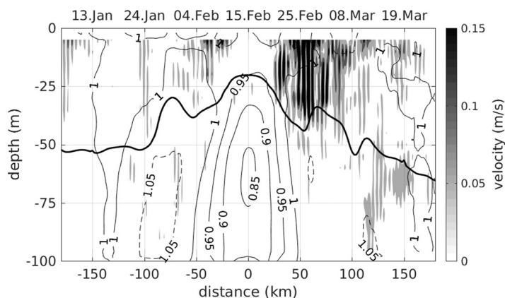
Figure 12. Near-inertial current amplitude ((u^2 + v^2)^{1/2}) at the mooring site calculated from band-pass filtered ADCP velocities from 10 January to 22 March 2010. Black contours represent f_{eff}/f . The thick black line shows the depth of the mixed layer.
