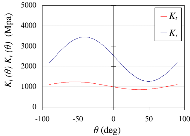
Figure 7. Analytical model of the specific cutting coefficients in relation to fibre orientation,
