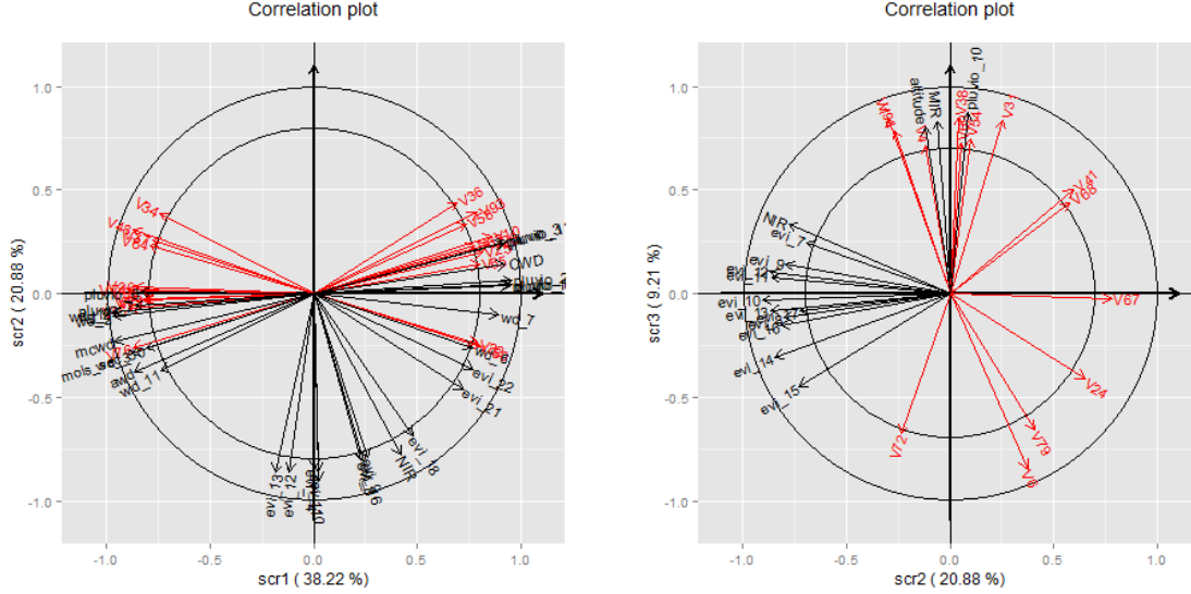
Figure 4: Two examples of correlations scatterplots on data Genus . The left hand side plot displays only variables having cosine greater than 0.8 with component plane (1, 2). It reveals two patterns: a “rain-wind”-pattern driven by the Pluvio’s and Wd’s variables and a photosynthesis-pattern driven by the Evi’s. On the right hand side, we plot variables having cosine greater than 0.7 with component plane (2, 3). Component 3 reveals a bundle driven by variables Altitude, MIR and Pluvio10, which prove important to model and predict several y ’s.
