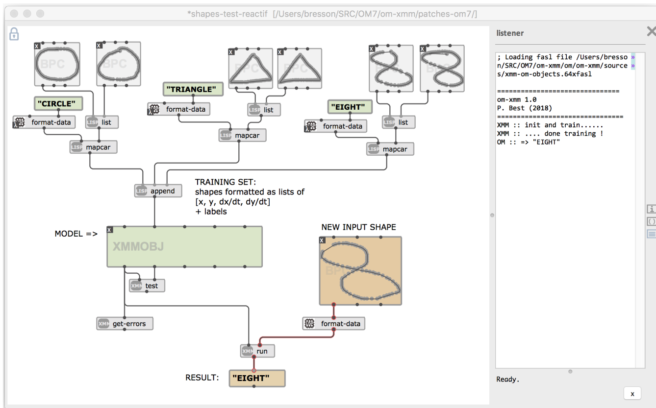
Figure 1: Basic shape recognition model using XMM in the OpenMusic visual programming environment. Using a small training set of [point-coordinates, class-label] , the model can estimate the class of a new input (hand-drawn shape at the right).
