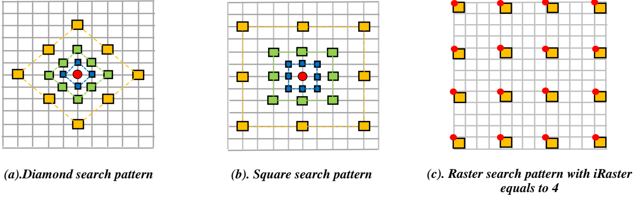
Figure 2. Diamond/Square/Raster search pattern
