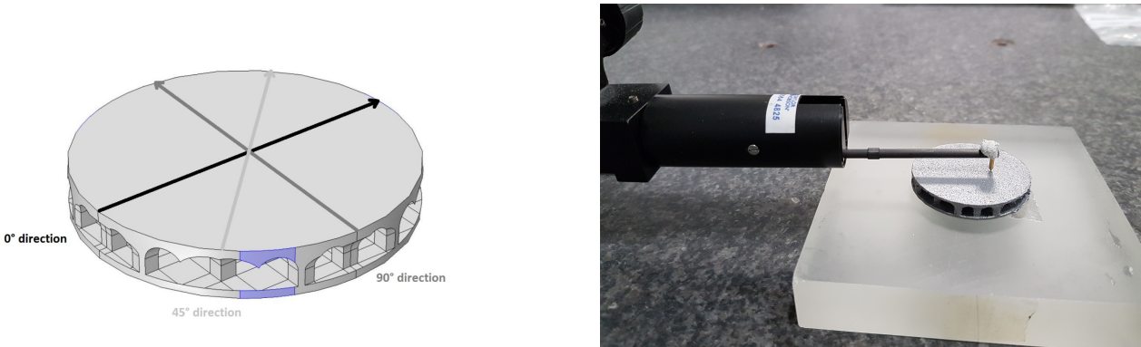
Figure 9. CAD view of the prototype design with the three direction measurements (left), Picture of the profilometry machine working on the AlSi10Mg raw sample (right)
