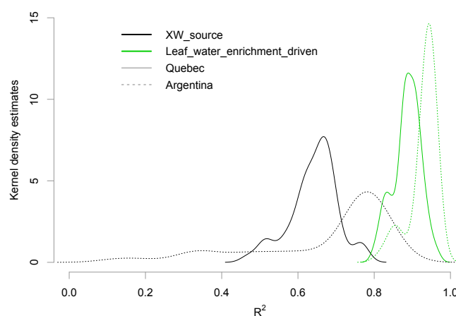
Figure 5. Density distributions of the coefficients of determination ( R^2 ) between the reference simulations and the (1) XW source experiment simulation ( \delta^{18}\text{O}_{\text{V}} and h_{\text{air}} set as constant, black) and (2) leaf water enrichment-driven experiment simulation ( \delta^{18}\text{O}_{\text{XW}} set as constant, green) in Québec (bold line) and Argentina (dashed line).
