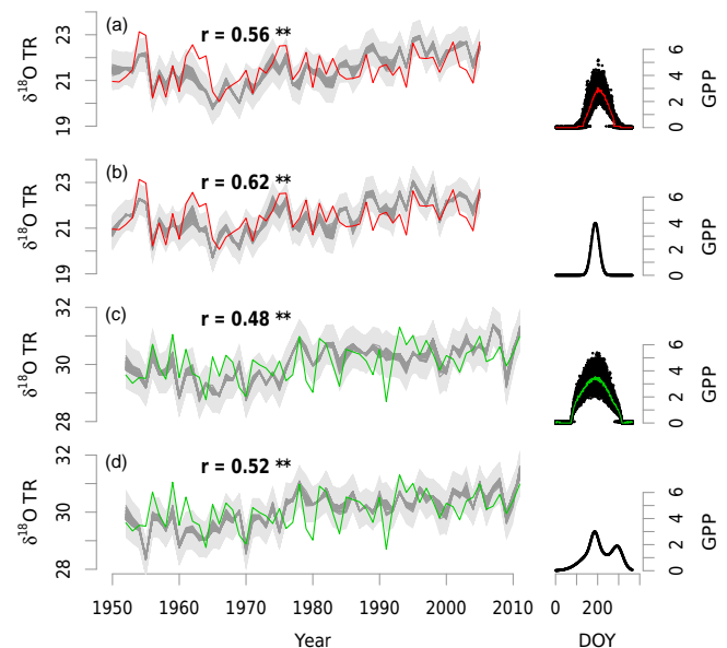
Figure 3. Comparison between observed (red or green) and simulated (grey) \delta^{18}\text{O}_{\text{TR}} chronologies in Québec (a and b) and Argentina (c and d), respectively, using GPP (in g C m -2 day -1 ) simulated by MAIDENiso for each day of the year (DOY) (a and c) or synthesized for maximizing correlations (b and d). The simulations are based on estimated \delta^{18}\text{O}_{\text{P}} series. The 50 different simulations inferred from the Markov chain Monte Carlo (MCMC) chains are in dark grey. The \pm 1 root mean square error (RMSE) range is represented in light grey. The mean correlation coefficients are significant at 99 % level (**).
