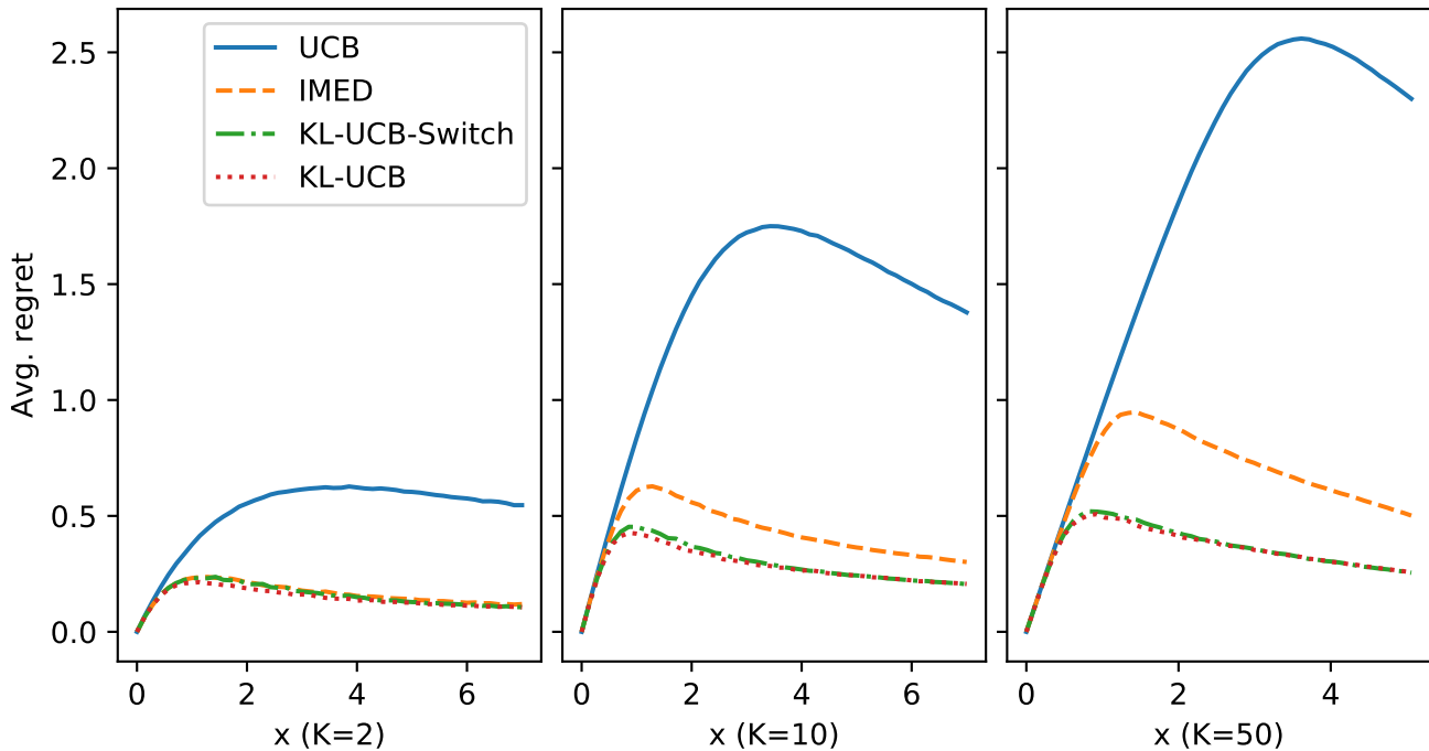
Normalized Average regret (Normalized for 5000 rounds), T=2000
