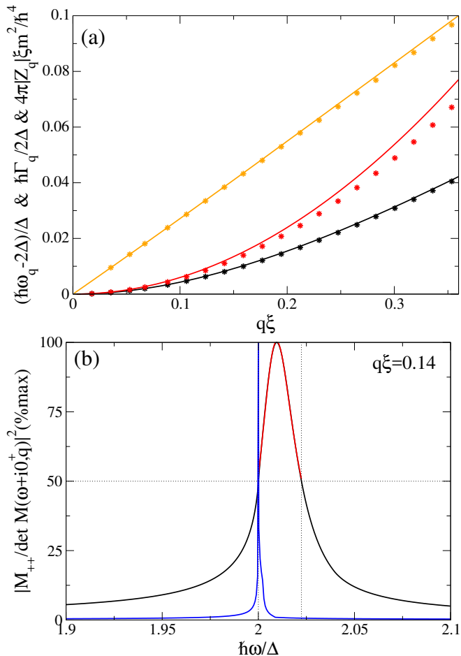
FIG. 5: (a) At weak coupling ( \Delta/\mu \rightarrow 0 ), frequency displacement \omega_{\mathbf{q}} - 2\Delta/\hbar , damping rate \Gamma_{\mathbf{q}} and residue Z_{\mathbf{q}} of the pair-breaking collective mode (black, red, orange solid lines) compared to the values (stars) extracted by fitting the amplitude response function 1/|M_{--}(\omega + i0^+, \mathbf{q})|^2 (black curve of (b)) by the function |C + Z_{\mathbf{q}}^{\text{fit}}/(\omega - \omega_{\mathbf{q}}^{\text{fit}} + i\Gamma_{\mathbf{q}}^{\text{fit}}/2)|^2 (red curve of (b)) describing a resonance on a flat background C . Blue curve of (b): amplitude response function |M_{++}/\det M(\omega + i0^+, \mathbf{q})|^2 at strong coupling ( \Delta/\mu = 10 ) exhibiting only a sharp peak at 2\Delta/\hbar .
