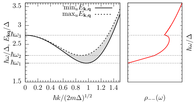
FIG. 1: Left: As a function of k , the interval between \min_u E_{\mathbf{k}\mathbf{q}} (reached for u = 0 , solid line) and \max_u E_{\mathbf{k}\mathbf{q}} (reached for u = \pm 1 , dashed line) determines an energy band (gray area) in which the resonance \hbar\omega = E_{\mathbf{k}\mathbf{q}} occurs for at least one value of u = \cos(\widehat{\mathbf{k}, \mathbf{q}}) in [-1, 1] . For fixed \omega , the integration interval over k in (6) is read horizontally; as a function of \omega , its structure undergoes 3 transitions in \omega_1 , \omega_2 and \omega_3 , which results in angular points in the spectral density. Right: Example of \rho_{--} (solid line). Here, \mu/\Delta = 1 and \hbar q/\sqrt{2m\Delta} = 0.5 .
