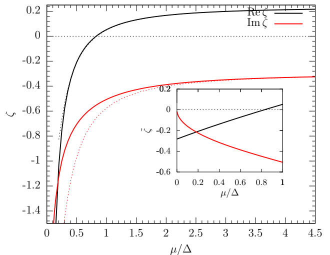
FIG. 4: Real and imaginary parts (black and red solid curves) of the dimensionless coefficient \zeta of q^2 in the energy z_{\mathbf{q}} of the pair-breaking collective mode as functions of \mu/\Delta . Dashed curves: weak coupling expansion \zeta = \zeta_0 - \frac{2\zeta_0^2}{\zeta_0 - 1} \left( \frac{\Delta}{\pi\mu} \right)^2 \ln^2 \frac{\Delta}{8\mu e} + \dots with \zeta_0 \simeq 0.2369 - 0.2956i . Inset: rescaled coefficient \tilde{\zeta} = \zeta\mu/\Delta = \zeta m/2m^* admitting the finite real limit \tilde{\zeta}_\infty = -16K^2(i)/\pi^4 \simeq -0.2823 at strong coupling \mu/\Delta \rightarrow 0^+ , its imaginary part tending to zero like -12K(i)(\mu/\Delta)^{1/2}/\pi^3 .
