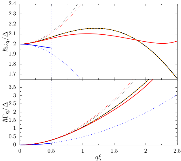
FIG. 3: Frequency (top) and damping rate (bottom) of the pair-breaking collective mode as functions of q for \mu/\Delta = 100 (black solid curve), \mu/\Delta = 5 (red solid curve) and \mu/\Delta = 0.1 (blue solid curve, disappears in 2k_0\xi \simeq 0.51 ) as functions of q in units of the inverse pair size \xi [2]. Dashed curves: the same for \mu/\Delta = 100 omitting the amplitude-phase coupling M_{+-} . Dotted curves: low- q quadratic behavior obtained analytically from Eqs. (10)-(14).
