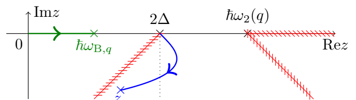
FIG. 2: Trajectories of the pair-breaking collective branch (blue curve) and Bogoliubov-Anderson branch (green line) as functions of q in the complex plane. The first one is revealed only after analytic continuation, hence the deformed branch cut (striped red lines) in the lower half-plane.
