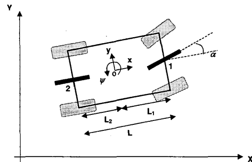
Fig. 1. Bicycle model.
