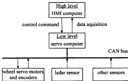
Fig. 5. Data transmission diagram.
