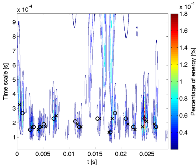
Fig. 6 Scalogram of the fluctuating pressure signal collected from probe 46. Crosses (x) indicate local pressure maxima and circles (o) indicate local pressure minima.
