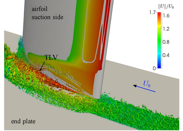
Fig. 4 3D instantaneous view of the zonal LES simulation. Isosurface of Q criterion, colored by the velocity magnitude.
