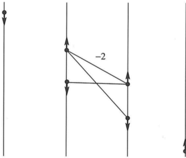
FIGURE 1. An abstract framed Morse complex
