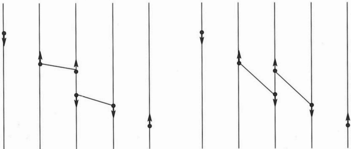
Its canonical form over \mathbb{Z}_2
