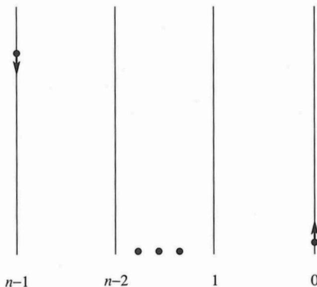
FIGURE 7. The abstract FMC of a linear function
