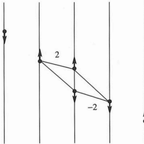
An abstract FMC
