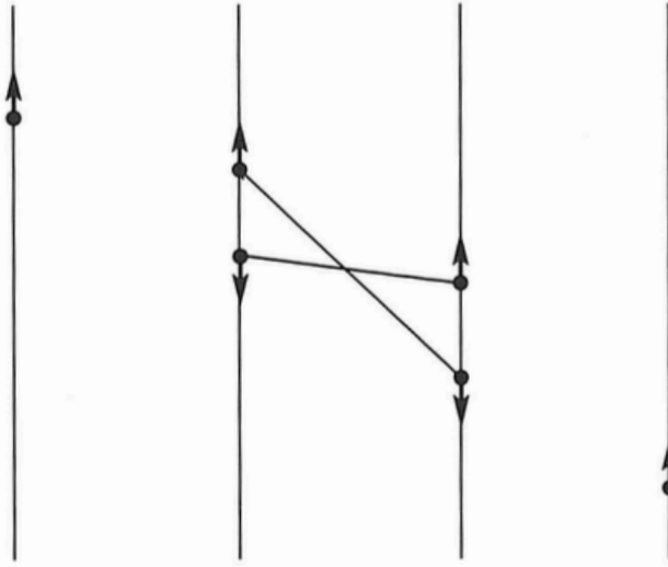
FIGURE 8. An abstract FMC having the simplest form
