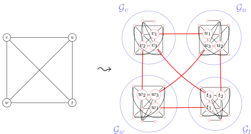
Fig. 2 Gadget associated to a vertex, u \in V with three neighbors v, w and t
