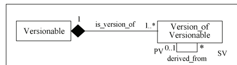
Fig. 2. Versioning Pattern
