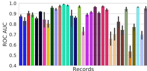
Fig. 3: ROC AUC scores (averaged) obtained on record-specific datasets of 1 s data segments using 5-fold cross-validation with the LR classifier.
