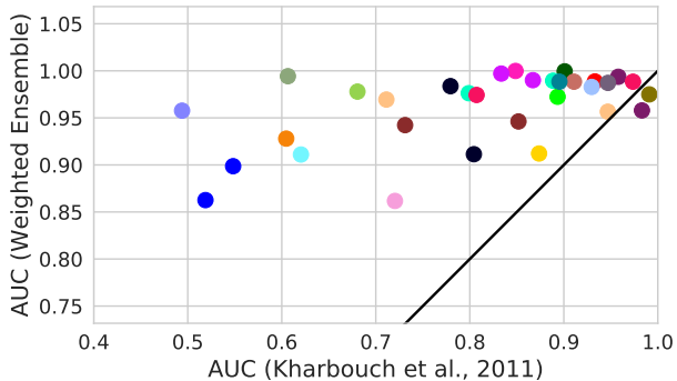
Fig. 1: Scatter plot of the ROC AUC scores (averaged) obtained on record-specific datasets of 5 s data segments using a 5-fold cross-validation. The solid black line represents the straight line joining the point (0, 0) to (1, 1).
