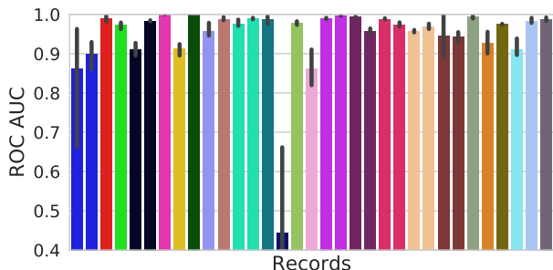
Fig. 2: ROC AUC scores (averaged) obtained on record-specific datasets of 5 s data segments using 5-fold cross-validation with the WE classifier. Each bar corresponds to an Epilepsiae record and adjacent bars of the same color correspond to records from the same patient.
