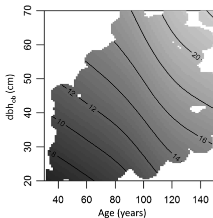
Fig. 4 Contour plot showing estimated double bark thickness in millimetres over age and breast height diameter outside bark ( dbh_{ob} ). Covariates that were included in the model but are not shown were set to the median of occurring values in the data. Shaded area approximately covers the region that was covered by observations
