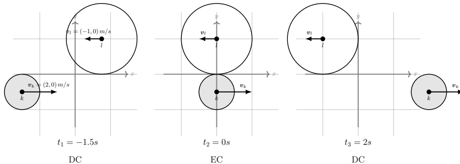
Fig. 1. An RCC story with three qualitative relations. Two circular entities k (radius = 1m ) and l (radius 2m ) moving with velocities \mathbf{v}_k = (2, 0) m/s and \mathbf{v}_l = (-1, 0) m/s in the interval [t_1, t_3] . The snapshots depict the temporal sequence of relations (DC, EC, DC) in the qualitative representation RCC (Fig. 3).
