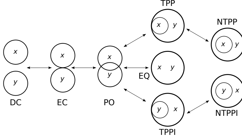
Fig. 3. The RCC qualitative relations depend on how two entities overlap. This Figure depicts the 8 RCC relations: DC, EC, PO, TPP, NTPP, EQ, TPPI, and NTPPI as a conceptual neighbourhood graph [11, 9]: the arrows connect relations that are conceptual neighbours [11] — we switch between conceptual neighbours by a continuous translation without going through any other relation.
