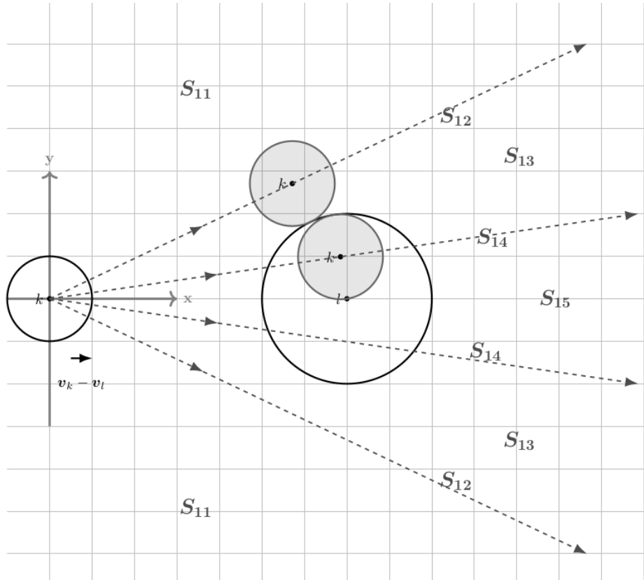
Fig. 4. In the representation RCC these are all the possible non-rigid stories, \Sigma_1 , i.e., the stories of two circles k and l moving in uniform motion with velocities v_k and v_l , so that v_k \neq v_l . The total number is five. Two stories are associated with directions: S_{12} = (\text{DC}, \text{EC}, \text{DC}) ; S_{14} = (\text{DC}, \text{EC}, \text{PO}, \text{TPP}, \text{PO}, \text{EC}, \text{DC}) . The remaining three stories are associated with the regions between the directions: S_{11} = (\text{DC}) , S_{13} = (\text{DC}, \text{EC}, \text{PO}, \text{EC}, \text{DC}) , S_{15} = (\text{DC}, \text{EC}, \text{PO}, \text{TPP}, \text{NTPP}, \text{TPP}, \text{PO}, \text{EC}, \text{DC}) . Note: The figure represents an equivalent simplification that considers l being motionless and k moving with the difference of velocities v_{kl} = v_k - v_l . The story depends on the direction of v_{kl} .
