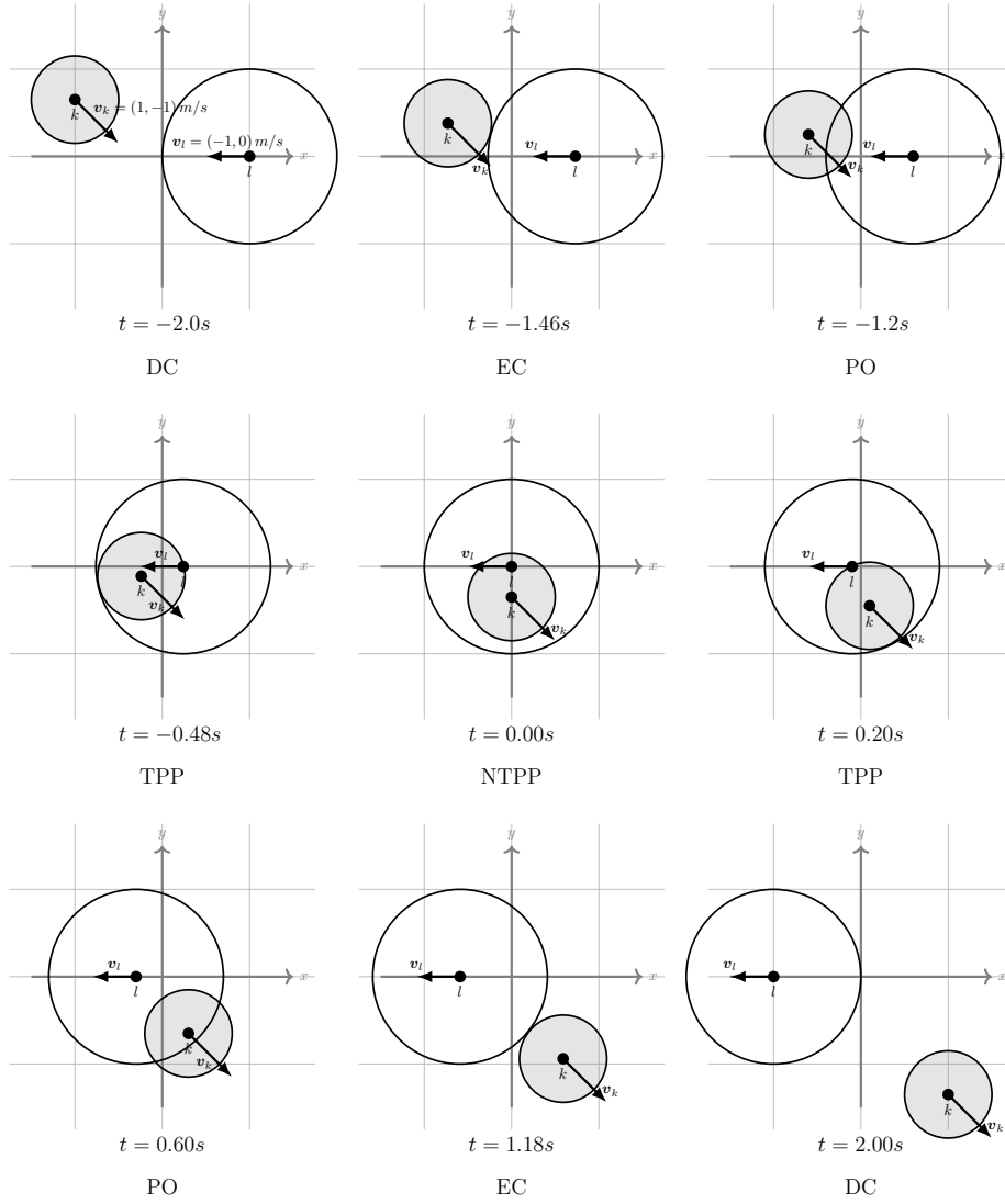
Fig. 2. A RCC story with nine qualitative relations. Two circular entities k (radius = 1m ) and l (radius 2m ) moving in uniform motion with velocities v_k = (1, -1) m/s and v_l = (-1, 0) m/s . They depict the Temporal Sequence of Relations (DC, EC, PO, TPP, NTPP, TPP, PO, EC, DC) in the qualitative representation RCC (Fig. 3). The snapshots correspond to different increasing times.
