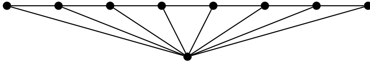
Figure 1: A fan on nine vertices.
