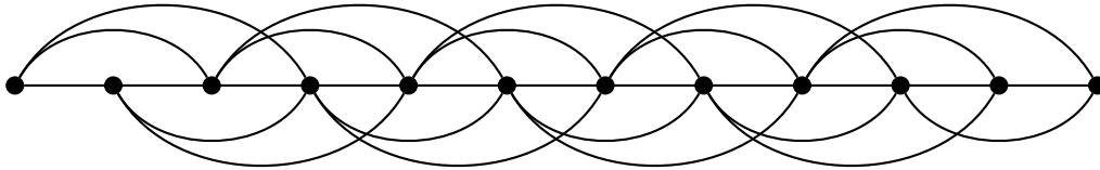
Figure 2: The graph P_{12}^3 .
