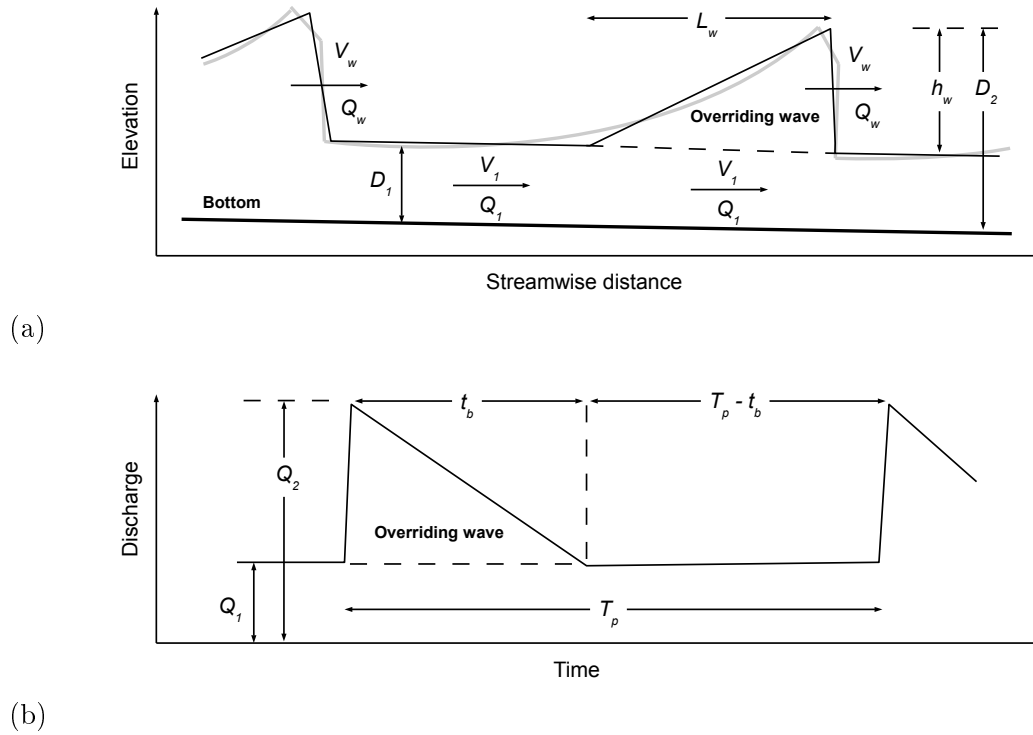
Figure 7: Schematic longitudinal elevation profile (a, modified after Thompson, 1968 ) and discharge time series (b) of a pulsated flow showing all useful variables for time-averaged discharge estimation. A more realistic profile of the roll waves is plotted in light gray (a, according to Brock's experiments reported by Richard and Gavriluk, 2012 ). D_1 , V_1 , Q_1 , are the depth, velocity, discharge, respectively, of the base flow. L_w , h_w , V_w , Q_w , are the length, height, mean velocity, mean discharge, respectively, of the surge. T_p is the time period between pulses, and t_b the transit time of pulse waves. The total flow depth at surge fronts, D_2 , is equal to D_1 + h_w . The total discharge at surge fronts, Q_2 , is considered over the full flow depth.
