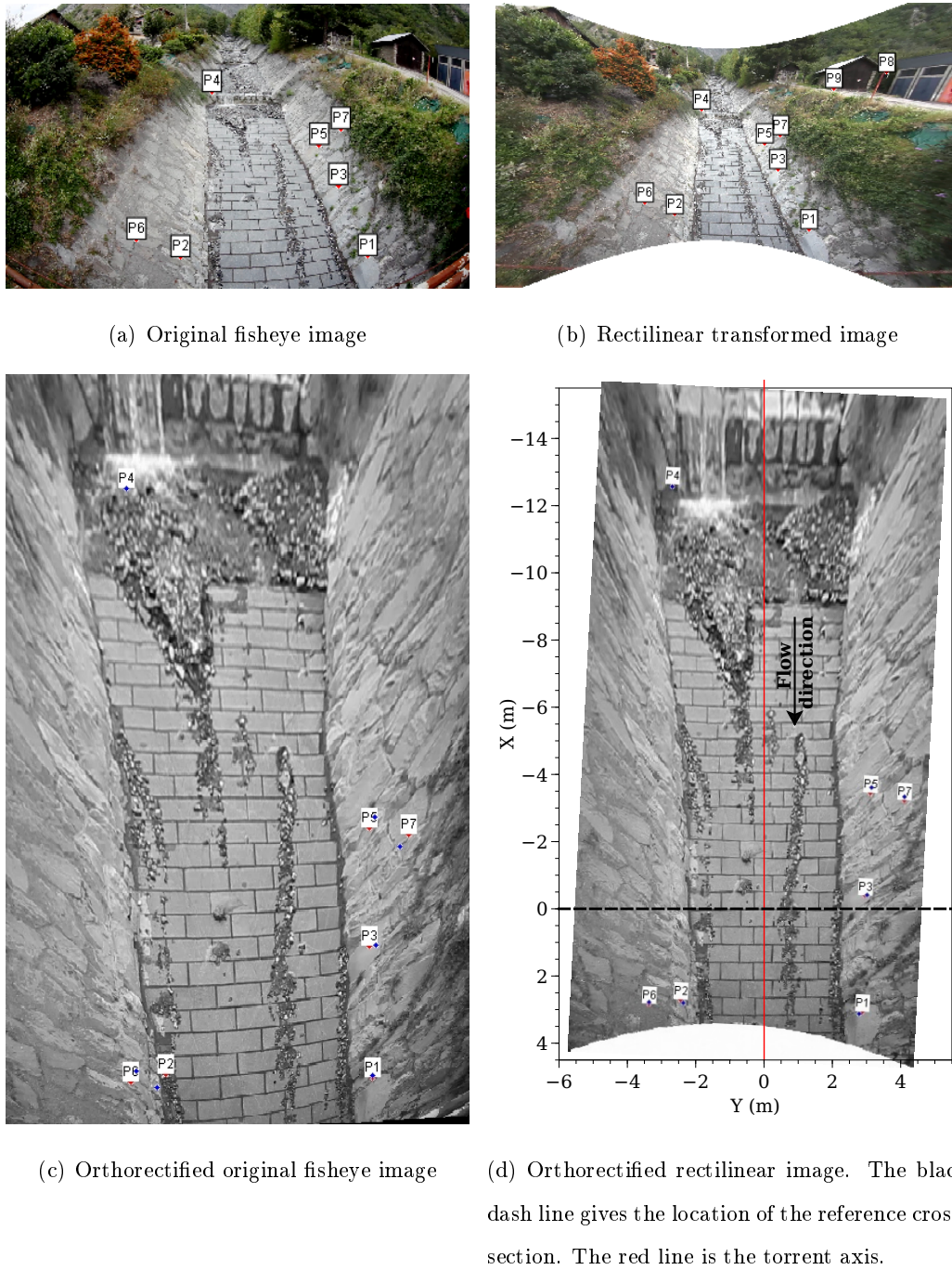
Figure 2: Comparison of original fisheye images and the same images corrected for distortion using rectilinear projection. The GRPs used for registration are displayed. Orthorectification is made in the plane of the torrent bottom.
