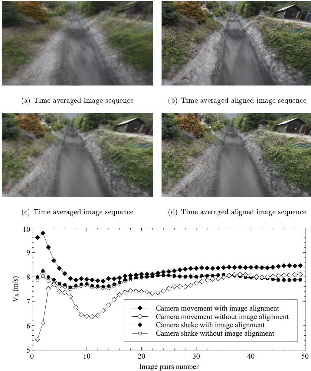
(e) Cumulative average values of streamwise velocity component, V_x , calculated at the reference cross-section with and without image alignment for the two types of movement
