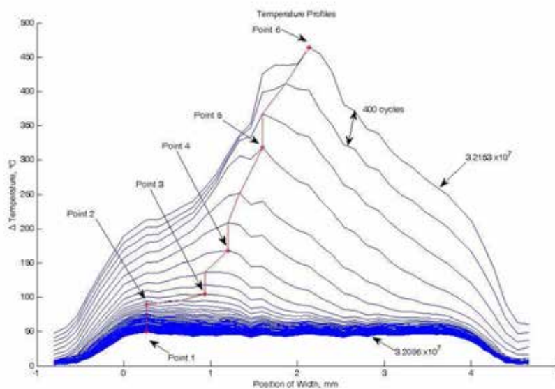
Figure 3 : Temperature profile along the specimen width
