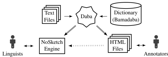
Figure 2: BRC data workflow
