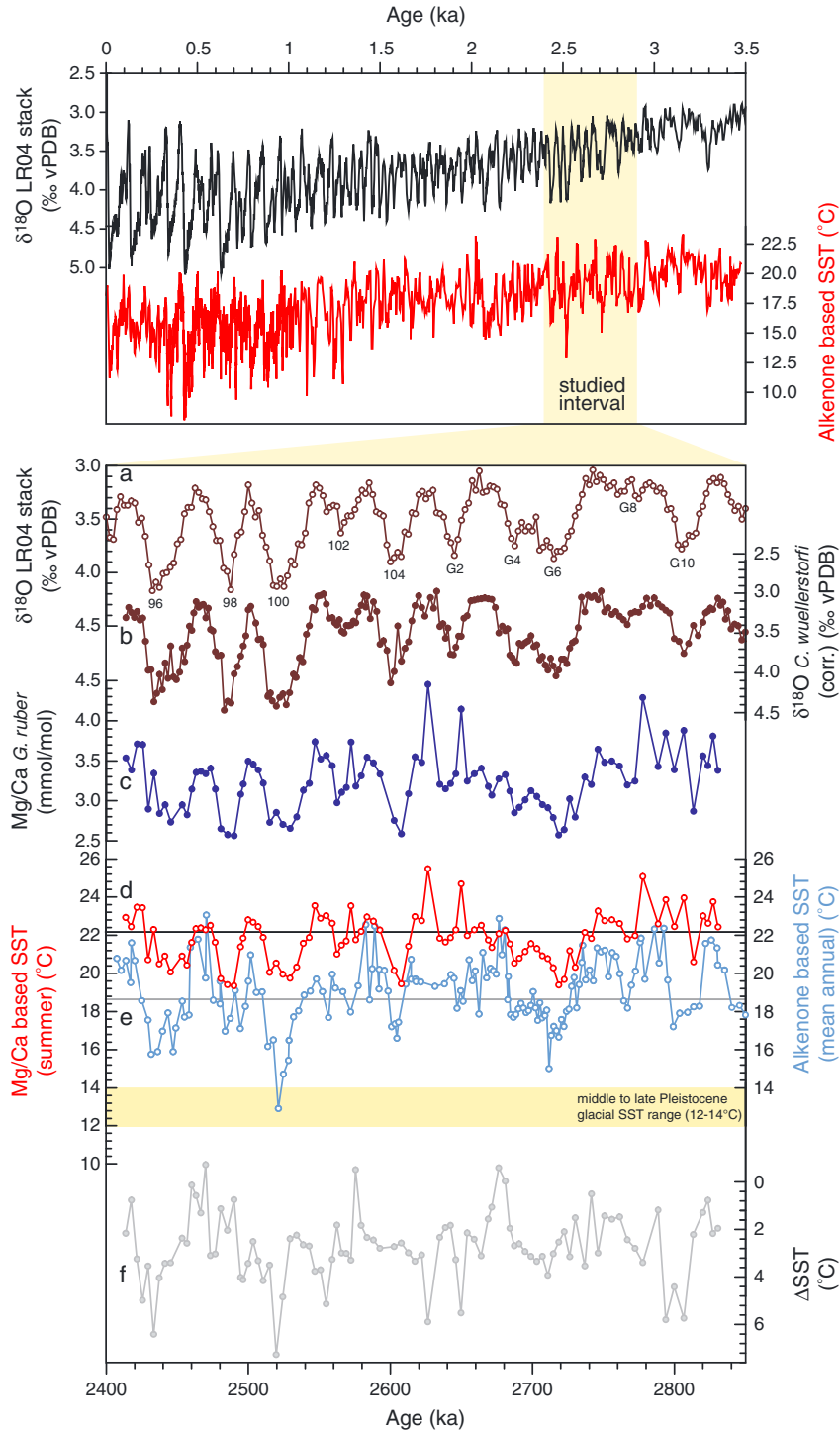
Figure 2. (top) Global benthic foraminiferal \delta^{18}\text{O} record (black) [Lisiecki and Raymo, 2005] and alkenone-based SST estimates from Site U1313 (red) [Naafs et al., 2012a] for the last 3.5 million years. (bottom) Orbitally resolved proxy records from Site U1313 for MIS G11 to 95 (2.9 to 2.4 Ma) tuned to the LR04 stack [Lisiecki and Raymo, 2005]. (a) The LR04 stack for MIS G11-95 [Lisiecki and Raymo, 2005]. (b) \delta^{18}\text{O}_{\text{benthic}} from Site U1313 [Bolton et al., 2010]. (c) Globigerinoides ruber Mg/Ca from Site U1313. (d) G. ruber Mg/Ca-based SST estimates from Site U1313. (e) Alkenone-based SST estimates from Site U1313 [Naafs et al., 2012a]. (f) Difference between Mg/Ca-based and alkenone-based SST estimates from Site U1313. Black and gray lines in Figures 2d and 2e represent modern mean summer (July, August, September (JAS)) and modern mean annual SST, respectively [Locarnini et al., 2006]. Pale yellow bar in Figure 2e represents range of alkenone-based SST estimates for middle to late Pleistocene glacials (without Heinrich event intervals) from Site U1313 for comparison [Stein et al., 2009; Naafs et al., 2012a].
