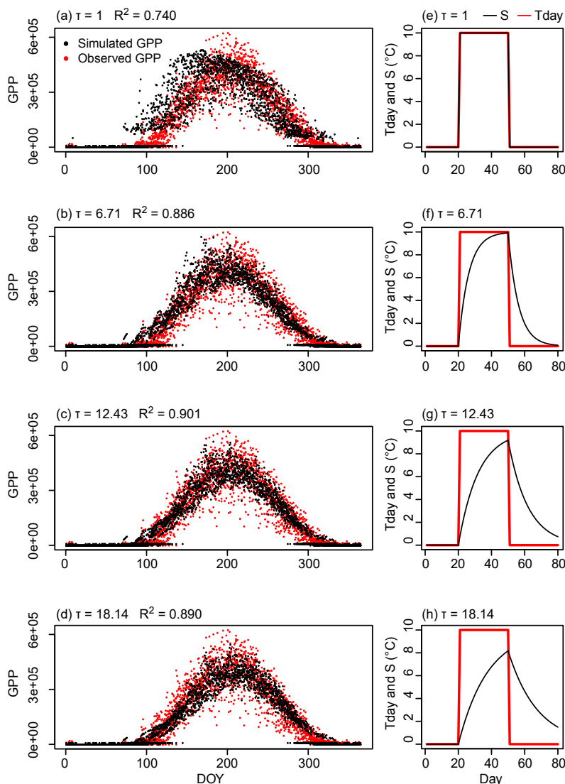
Figure 6. Influence of the temperature transformation ( S ) on the modeled annual cycle of GPP daily values ( \mu\text{mol C m}^{-2} \text{ day}^{-1} ) at the Quebec Eastern Old Black Spruce site. Only the \tau parameter determining the S values was allowed to vary, while the other parameters were fixed to the values of plausible block GPP. (a) \tau is 1 day ( S same as Tday). (b) \tau is 6.71 days (a middle value between 1 and 12.43). (c) \tau is 12.43 days (same \tau than in plausible block GPP). (d) \tau is 18.14 days (a higher value than in plausible block GPP). The R^2 between observations and simulations is reported in each plot. Panels (e–h) show the impact of the respective \tau values on S if the daily Tday time series corresponds to a single step of 10 °C lasting 30 days.
