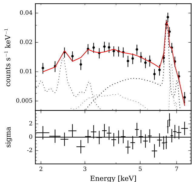
Fig. 3. Spectrum of Sgr C1 observed with EPIC-pn onboard XMM-Newton in 2012. The red line corresponds to the best-fit model. The dotted lines show the three components of the model: the hot ( thin line ) and soft ( medium ) thermal plasmas, and the Monte Carlo reflected emission ( thick ).
