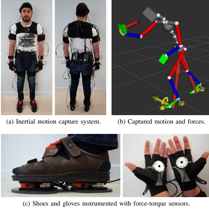
Fig. 2. Acquisition system for whole-body kinematics and contact forces.
