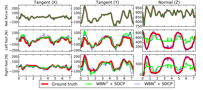
(a) Two contacts: upper-body balancing with static feet.
