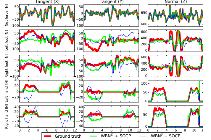
(c) Four contacts: leaning against a wall with two hands at the same time.
