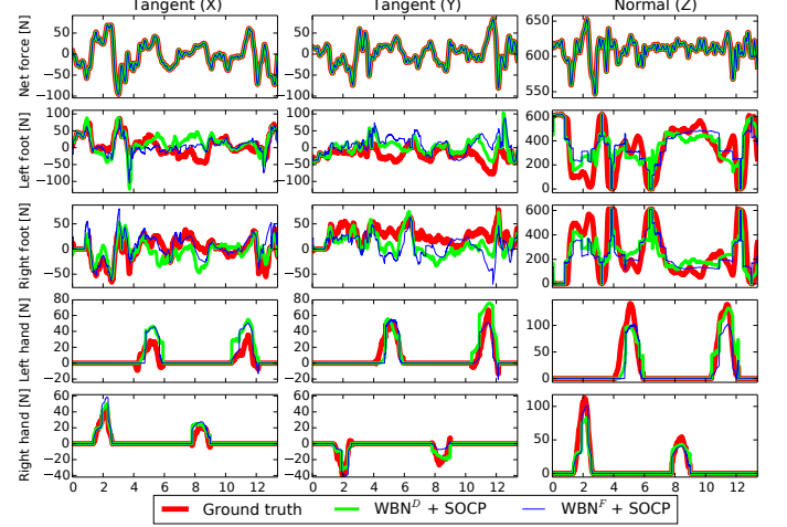
(b) Three contacts: taking support on a table with one hand (alternating).
