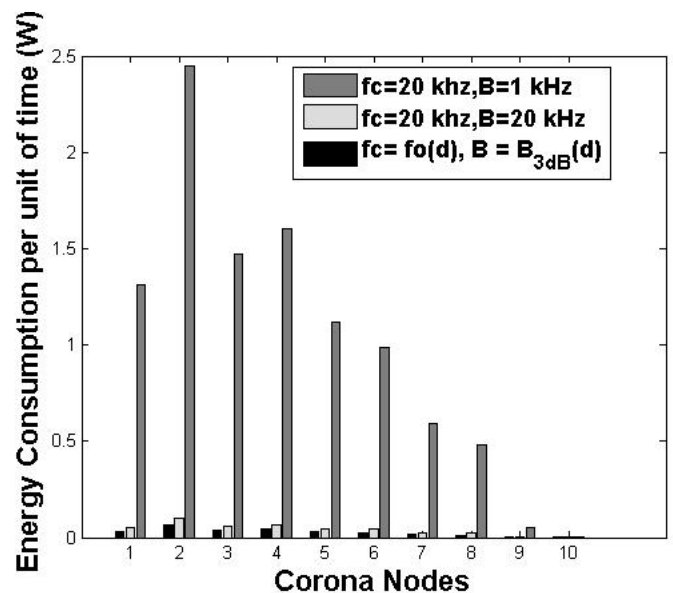
Fig. 18. Energy Consumption per corona for various frequency band.
