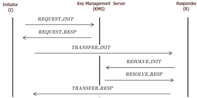
Figure 1: MIKEY-Ticket full three round-trip mode exchange (RFC 6043)
