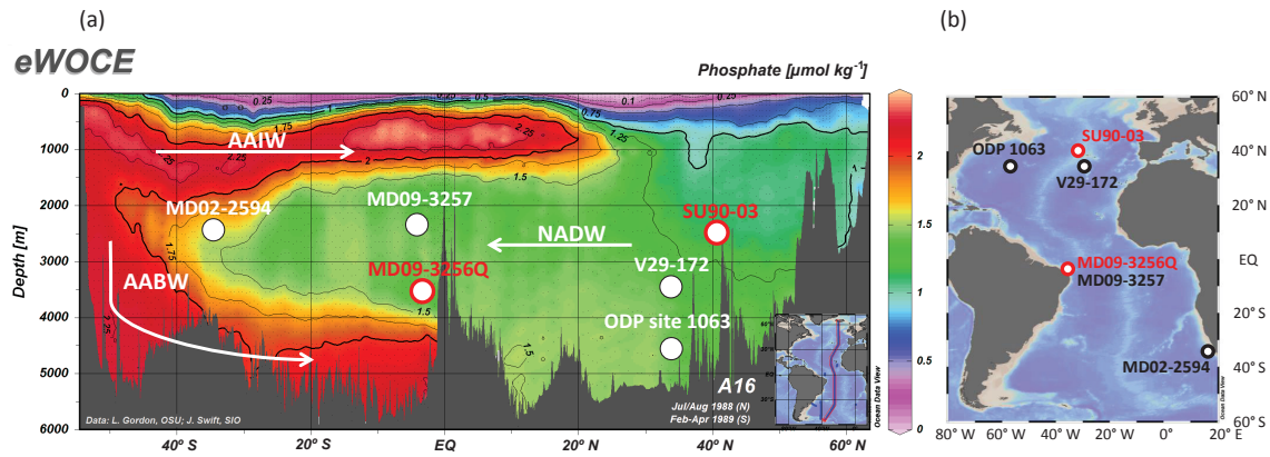
Figure 1. (a) Phosphate section (Schlitzer, 2000) and (b) map of the Atlantic Ocean showing the location of the studied sediment cores (see Sect. 2.1 or Table S1 for detailed locations). Cores, for which we provide new Pa / Th or \delta^{13}\text{C} data, are circled in red. Phosphate content follows the structure of the present-day AMOC. White arrows indicate the approximate flow directions of the Antarctic intermediate water (AAIW), Antarctic bottom water (AABW) and North Atlantic deep water (NADW).
