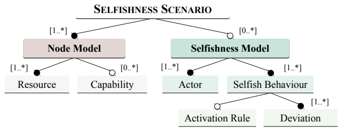
Fig. 2: Feature diagram of a selfishness scenario.
