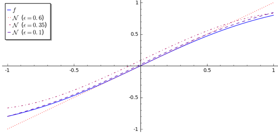
FIGURE 5.2. The graphs of f(x) = 4x/(4 + x^2) and some of its approximators ( \lambda = 1/4 )
